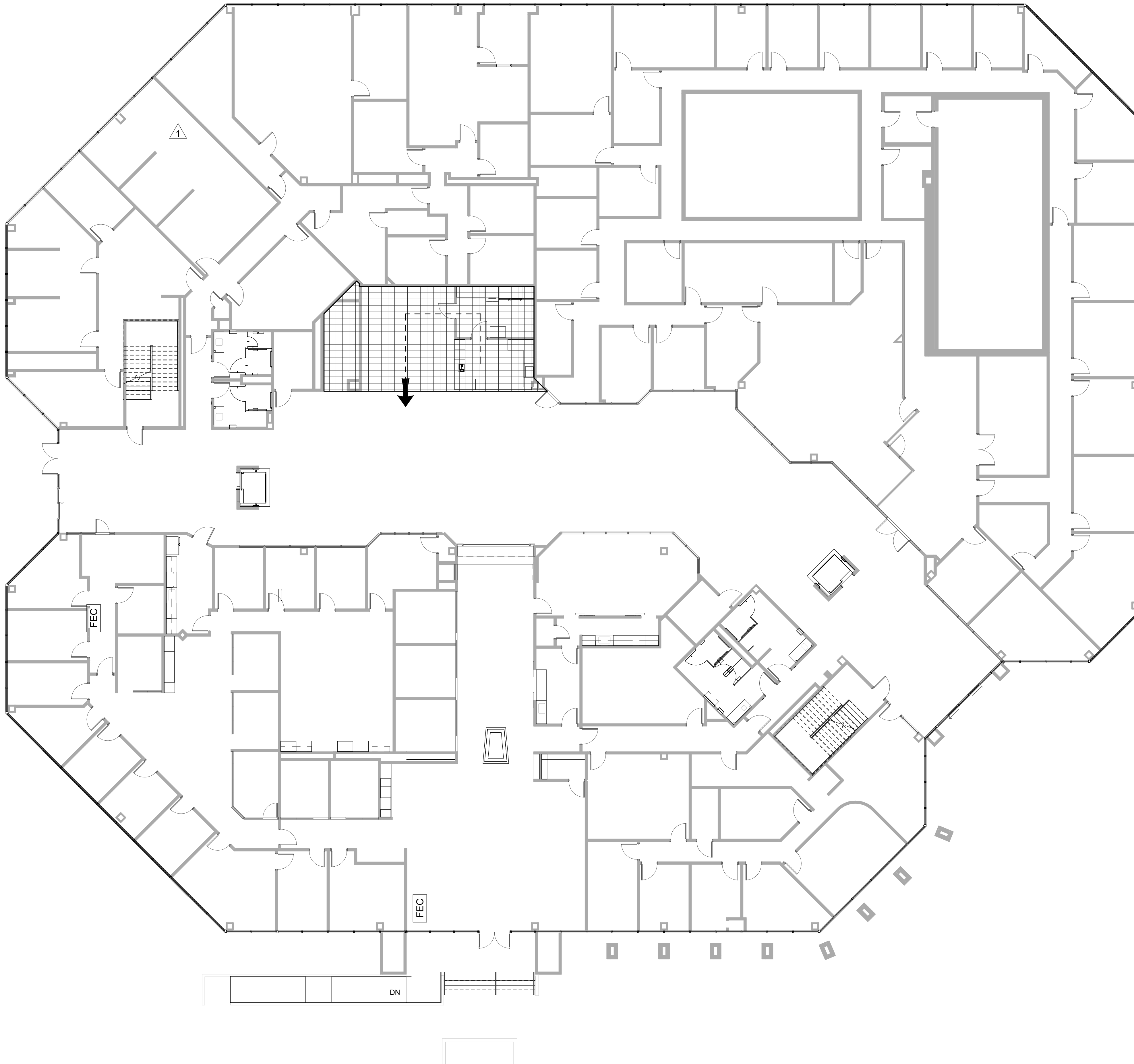
A1 OVERALL LIFESAFETY PLAN 3/32" = 1'-0"
