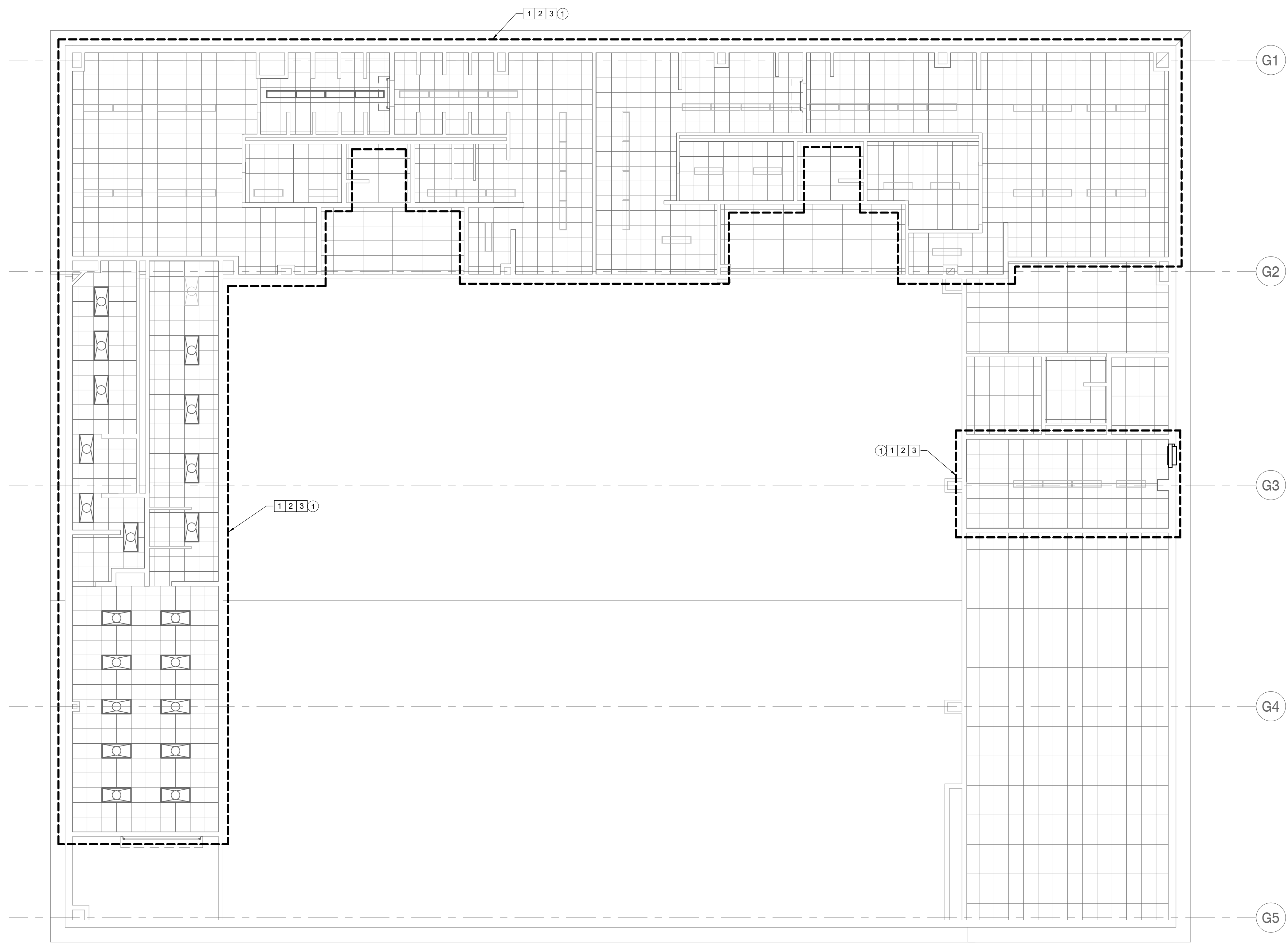
1 MECHANICAL ELECTRICAL PLAN - GYMNASIUM BUILDING ME2.04 1/8" = 1'-0"
